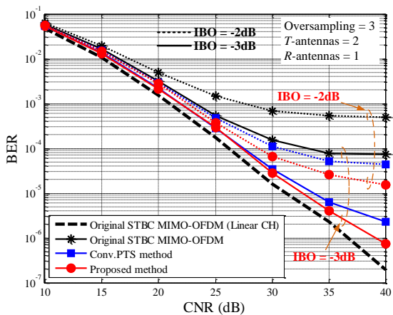
Figure.9 BER vs. CNR(dB)
