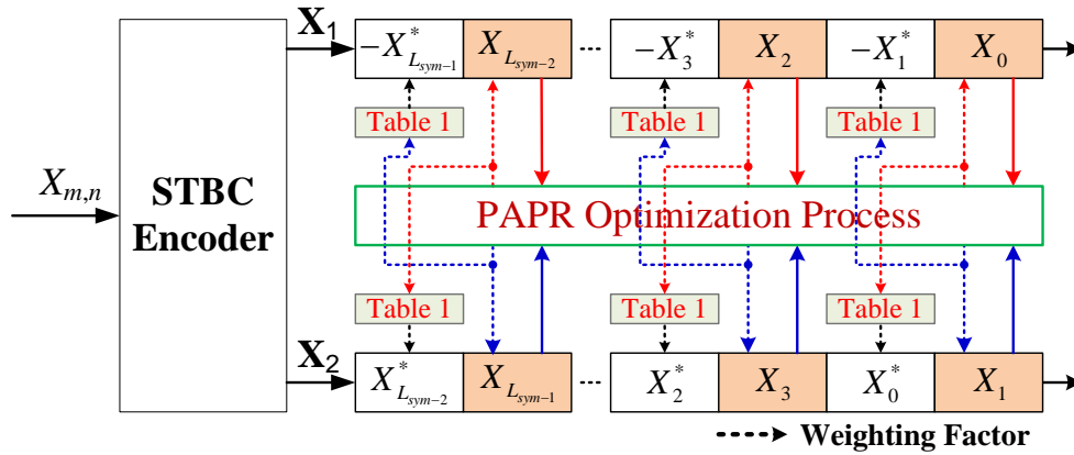
Figure.5 PAPR reduction with concurrent algorithm
