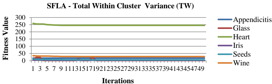
Fig. 2 Result for proposed SFLA algorithm using TW Fitness Function
